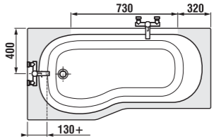
These areas are recommended for placing a bathtub outlet or a bathtub mixer outlet.
